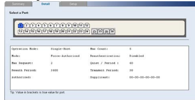
Figure 58 802.1X Detail Screen
